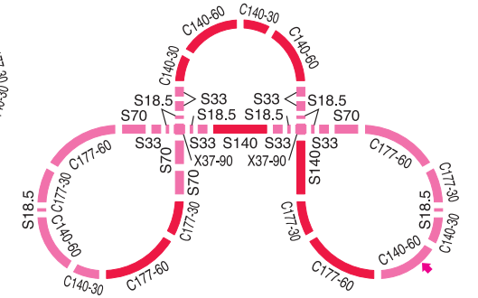
MA+MX+MX 579×914mm
