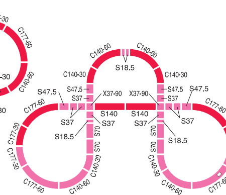
MA-WT+MX-WT+MX-WT 597×951mm
