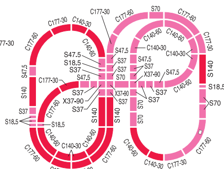
MA-WT+MA-WT+MX-WT+MX-WT+MX-WT 690×778mm
