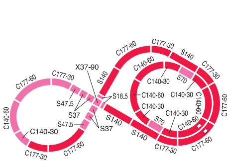
MA-WT+MA-WT+MX-WT 452×922mm
